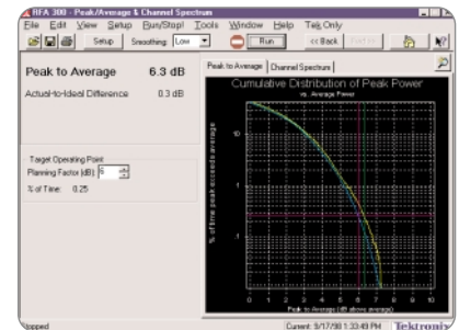
► Peak to Average Power and Actual-to-Ideal Difference with Cumulative Distribution of Peak Power and Channel Spectrum Graphics.
